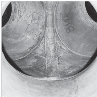
KALSICA lined pipe transition
